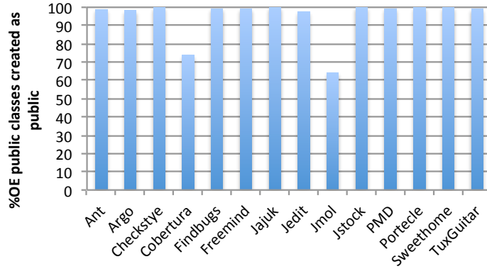
Figure 4: Analysis of the creation of over-exposed public classes
