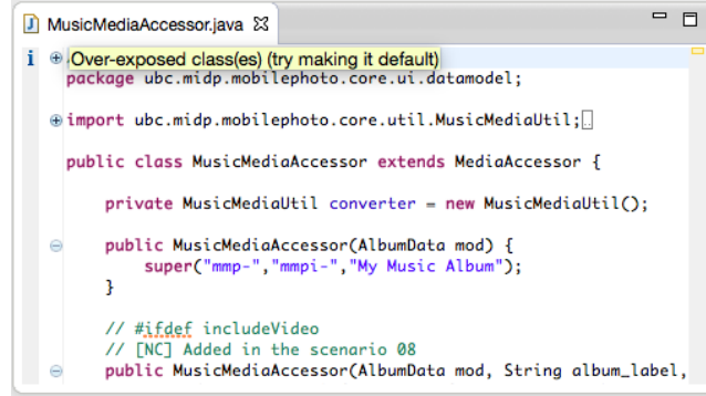
Figure 7: Refactoring suggestion of Cover
