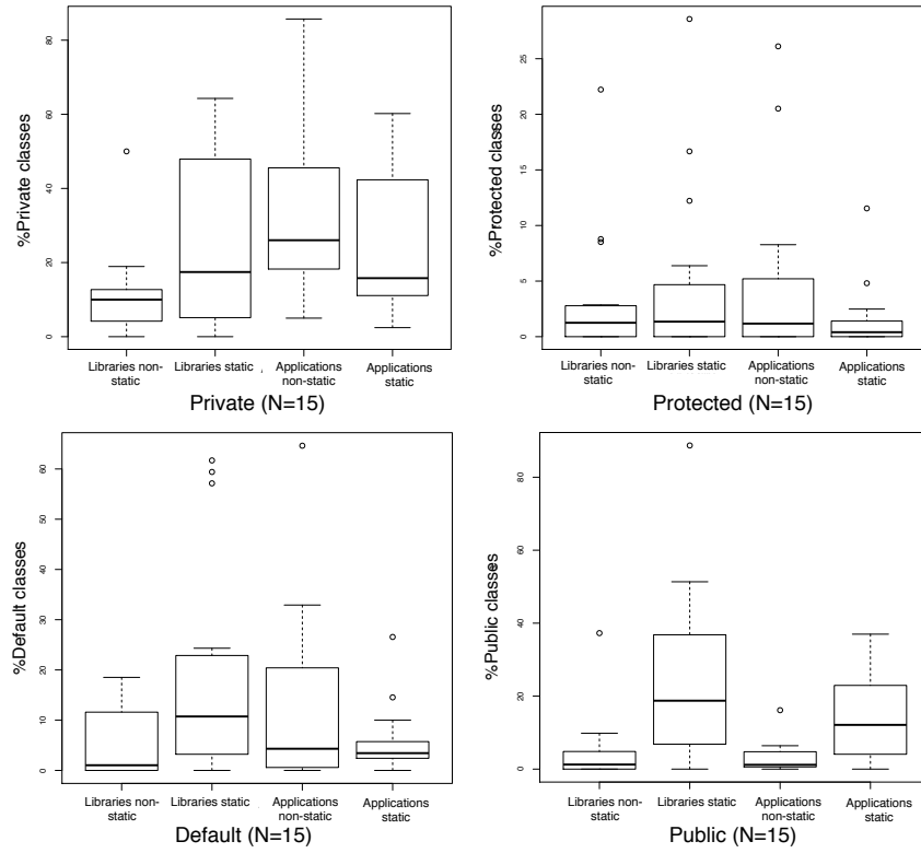
Figure 2: Distribution of nested classes accessibility
