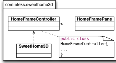
Figure 3: Example of over-exposure in class HomeFrameController
